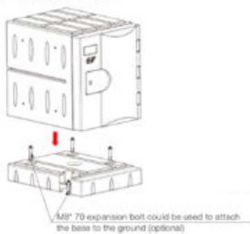
Schematic diagram with ground
