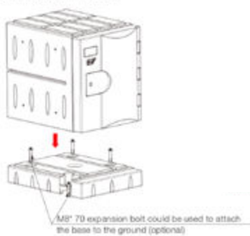
Schematic diagram with ground
